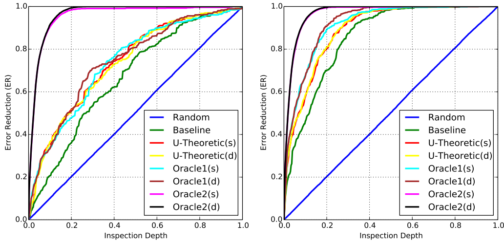
Fig. 3. Results obtained by (a) splitting the REUTERS-21578 test set into 10 random, equally-sized parts, (b) running the analogous experiments of Figure 2 independently on each part, and (c) averaging the results across the 10 parts. The learners used are MP-BOOST (left) and SVMs (right).
