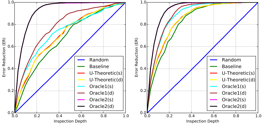
Fig. 4. Same as Figure 3 but with REUTERS-21578/100 in place of REUTERS-21578/10. The learners used are MP-BOOST (left) and SVMs (right).
