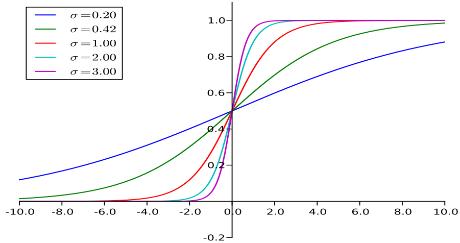
Fig. 1. The generalized logistic function.
