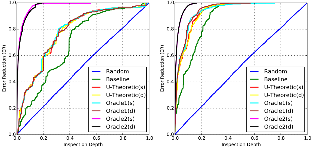
Fig. 2. Error reduction, measured as ER_\rho^M , as a function of validation depth. The dataset is REUTERS-21578, the learners are MP-BOOST (left) and SVMs (right). The Random curve indicates the results of our estimation of the expected ER of the random ranker via a Monte Carlo method with 100 random trials. Higher curves are better.
