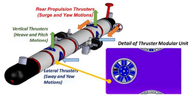
Fig. 2. MARTA AUV, division in modules and propulsion system
