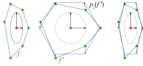
Figure 7: A single face f of the ACVT with the eigenvectors resulting from PCA (left); the un-stretched polygon f' with the aligned target polygon p_t(f') (middle); and the computed displacement vectors in the original space (right).
