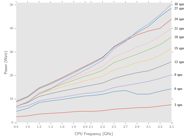
Figure 1: Average operational power (measured in Watts) consumed by a query server at different CPU frequencies and different workloads.
