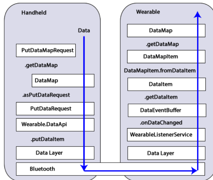
Figure 10 The PutDataMapRequest helper class simplifies the process of creating the DataMap , DataItem , and PutDataRequest objects that are needed for sending data. On the receiving side a WearableListenerService receives changed data and returns a buffer of DataEvents containing DataItem to be converted into DataMapItem containing the original handheld data
