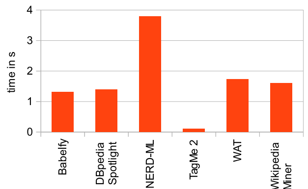
Figure 4: Runtime per document of different approaches in GERBIL for the A2KB experiment type on the MSNBC dataset.
