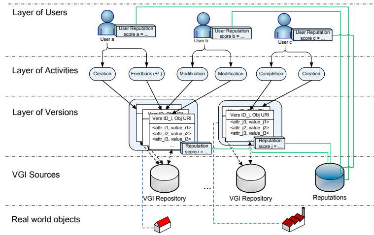
Fig. 1. Reference multi-layer architecture for VGI reputation.
