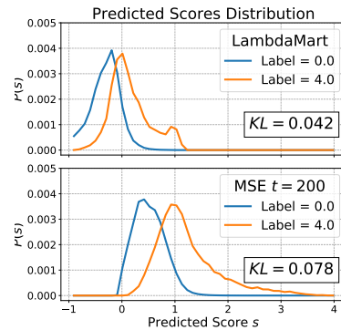
Figure 2: Discriminative power after 100 trees. Predicted score for documents with largest and smallest label.
