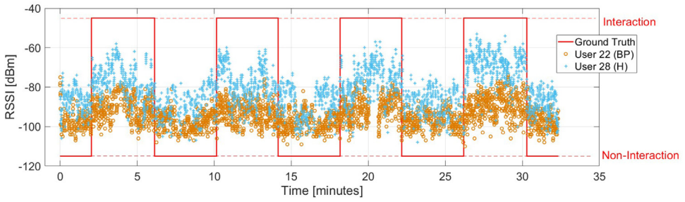
Fig. 5. Example of raw data of RSSI values from dyad 22 and 28 during Session 5, Test 1.
