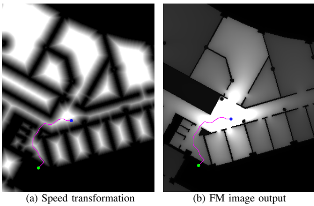
Fig. 4. FM examples. Blue and green dots represent origin and destination points, respectively. Magenta lines show the paths determined applying FM.
