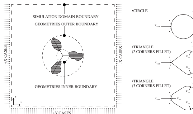
Figure 9: 2D CFD analysis method: analysis domain and explored shape options
