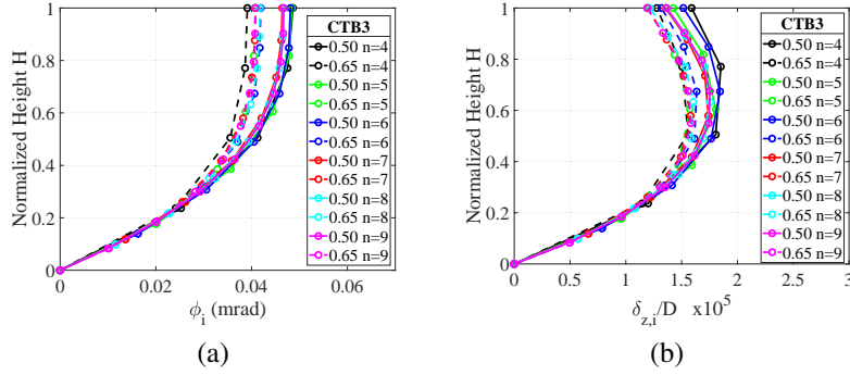
Figure 14: Bundling effect for the H = 320\text{ m} model (aspect ratio set to 1:4, bamboo model limit set to 0.50 and 0.65): (a) rotations; (b) maximum vertical displacement.
