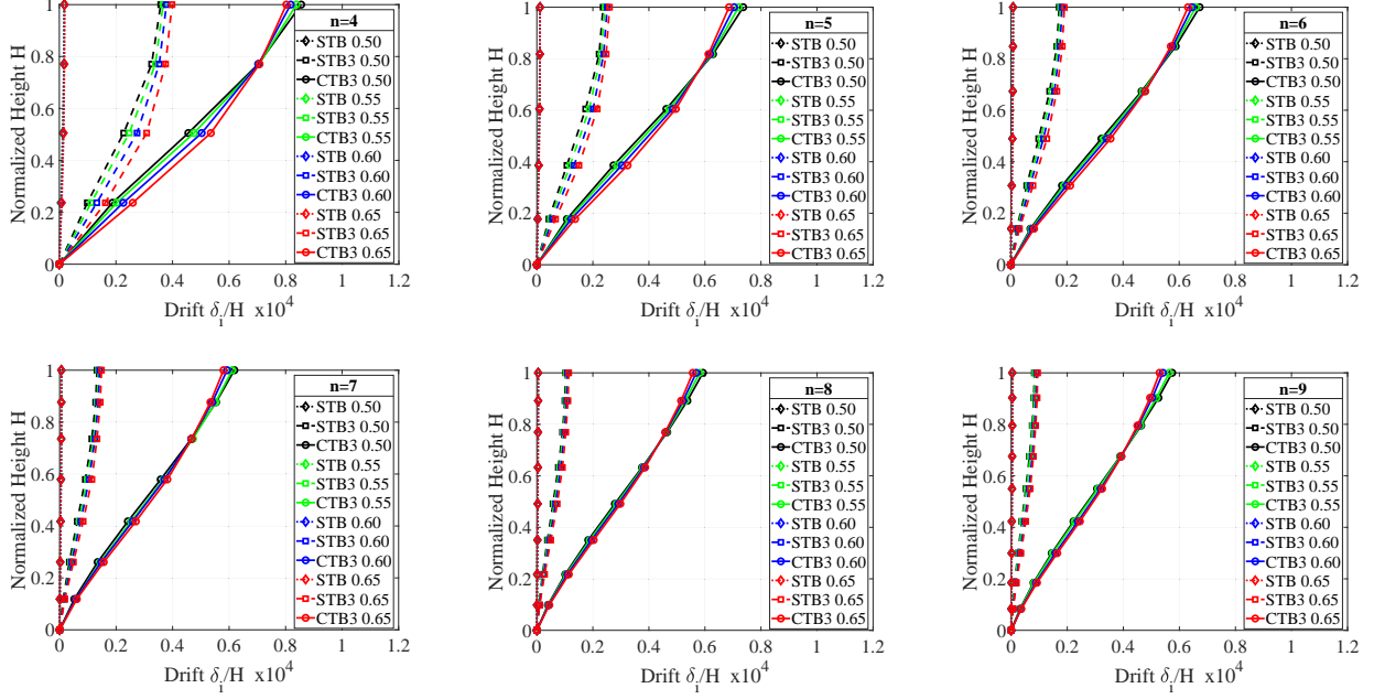
Figure 13: Bundling effect for the H = 320\text{ m} model (aspect ratio set to 1:4).
