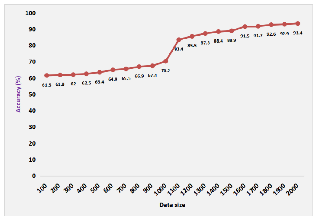
Figure 9. Sensitivity analysis with respect to the data size using CBECS dataset samples.
