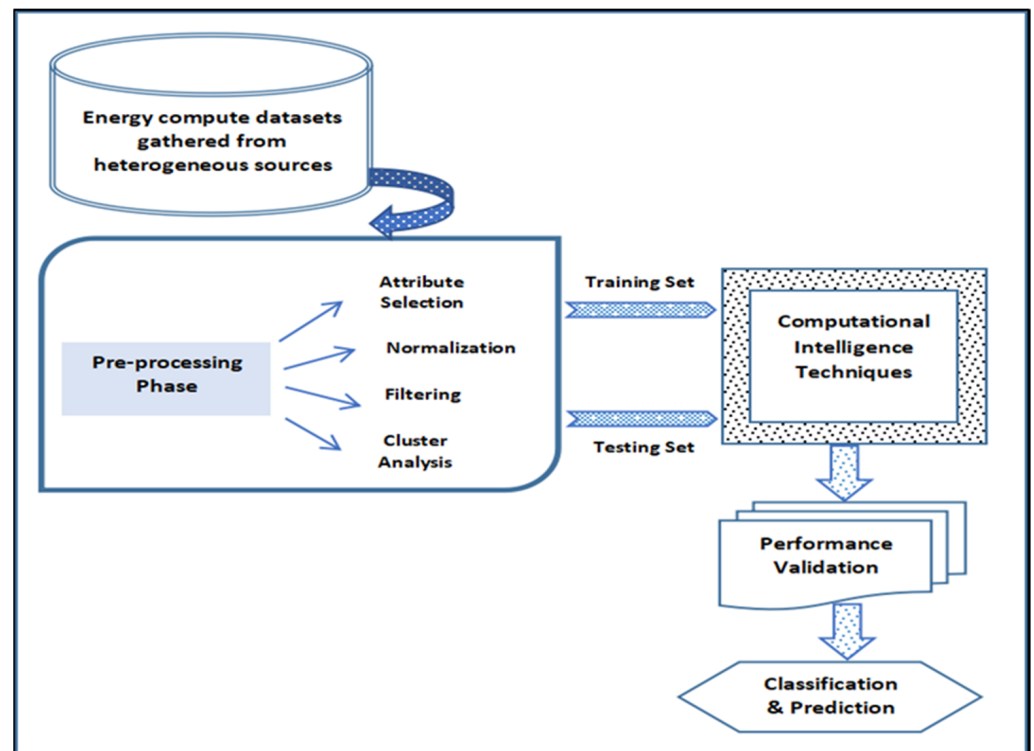
Figure 1. A generalized computational intelligence model for energy consumption analysis.
