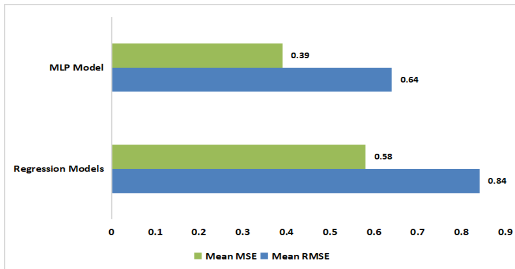
Figure 8. Error rate analysis with MLP and other regressor models using the CBECS dataset.
