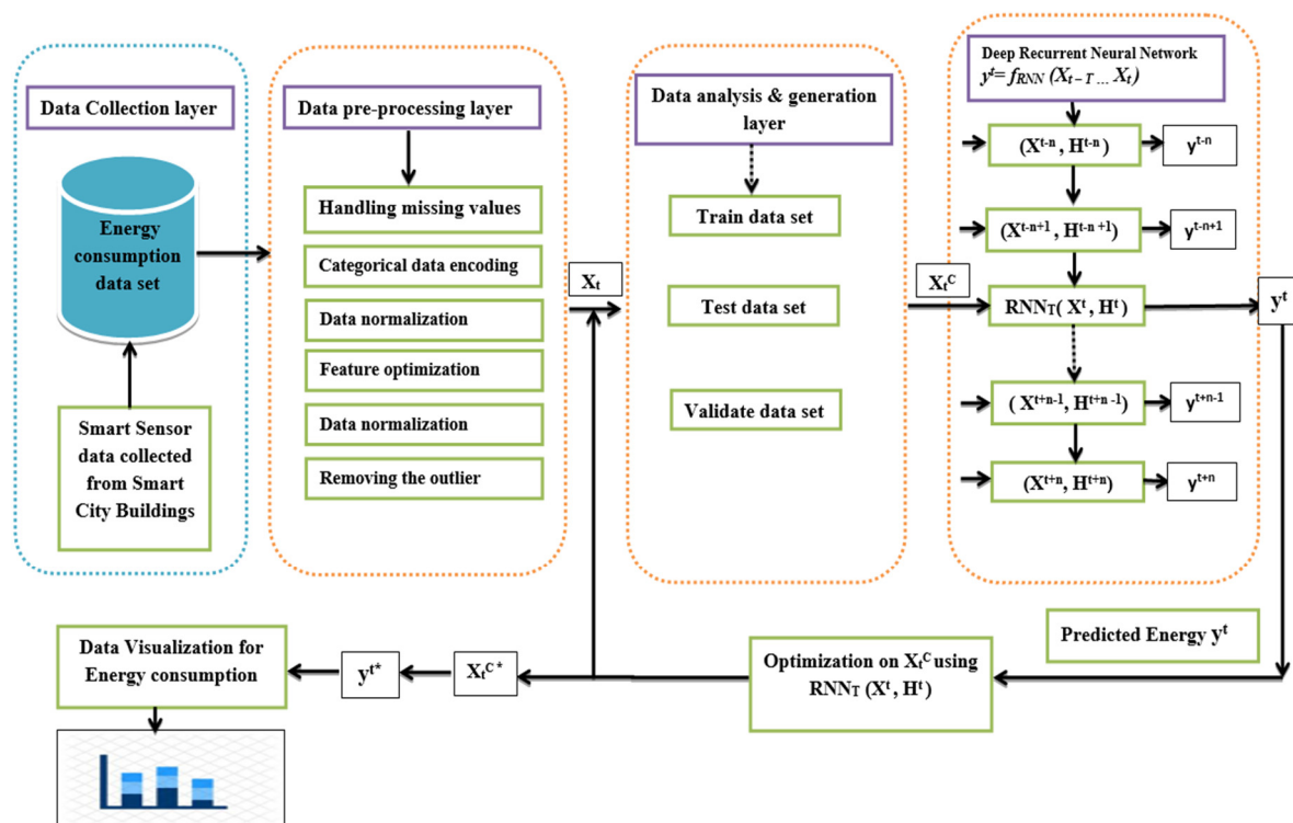
Figure 11. A deep neural network-enabled energy consumption model for smart city buildings.
