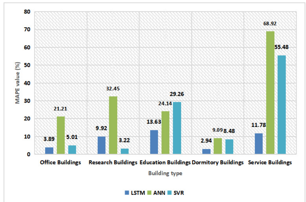
Figure 7. MAPE value for different buildings using LSTM, ANN and SVR models for energy utilization.
