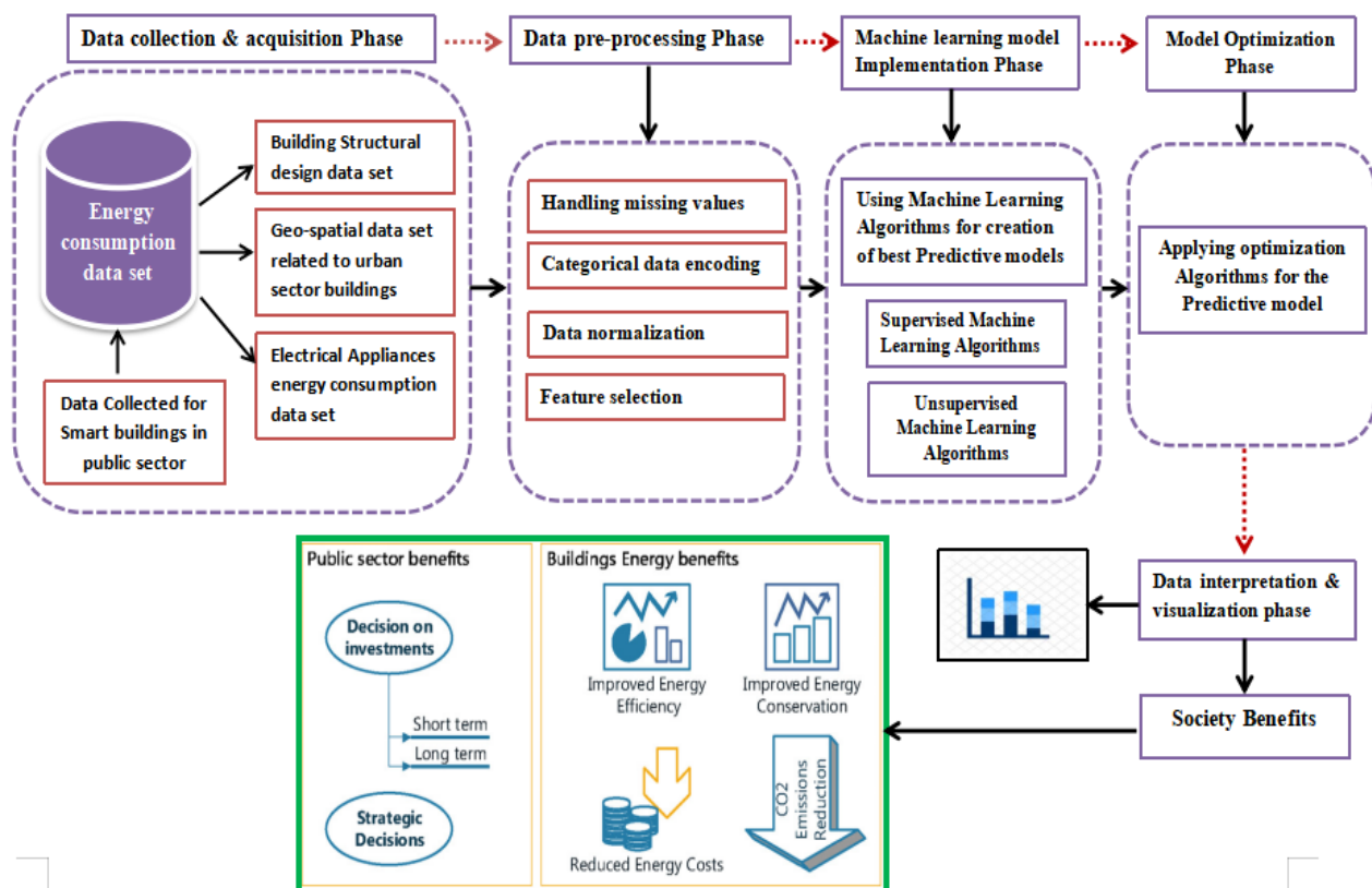
Figure 10. A multi-purpose predictive model for energy efficiency computation in the urban sector.
