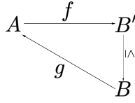
Figure 1: Graphical representation of \mathcal{I} \Vdash A \Rightarrow B .
