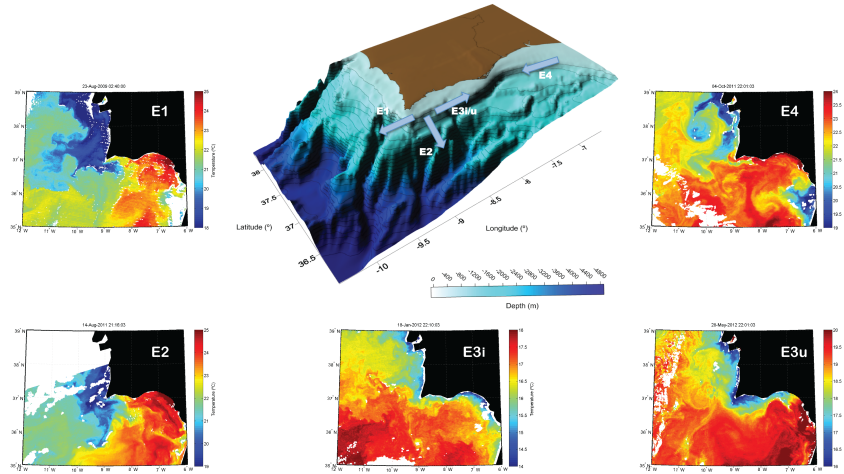
Figure 1. Mesoscale patterns in the south-western Iberian Peninsula (from [13]).
