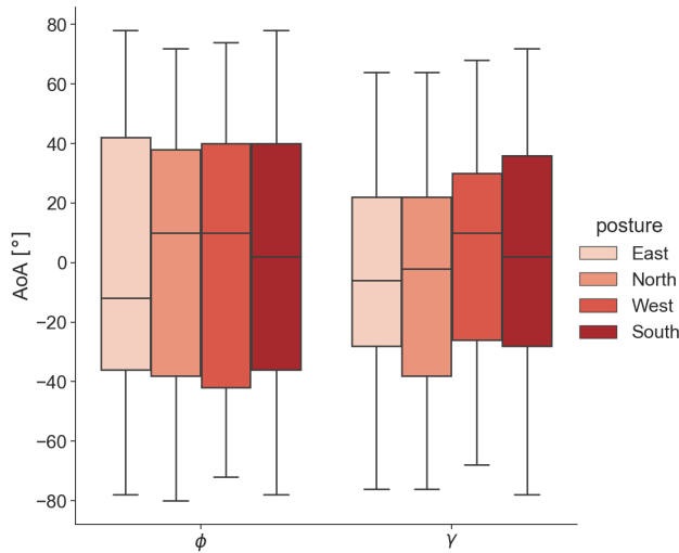
Fig. 12: AoA distribution for different postures and angles.
