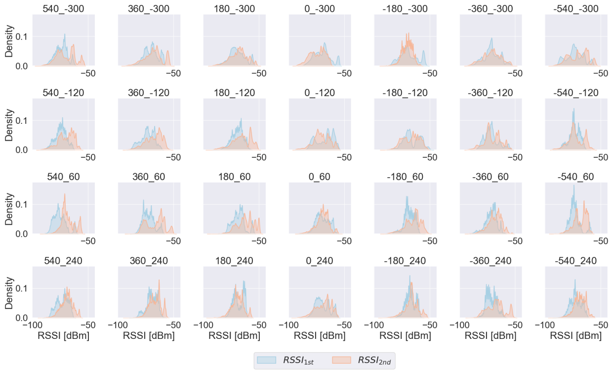
Fig. 8: RSSI distribution on 1st and 2nd polarization for 28 locations.
