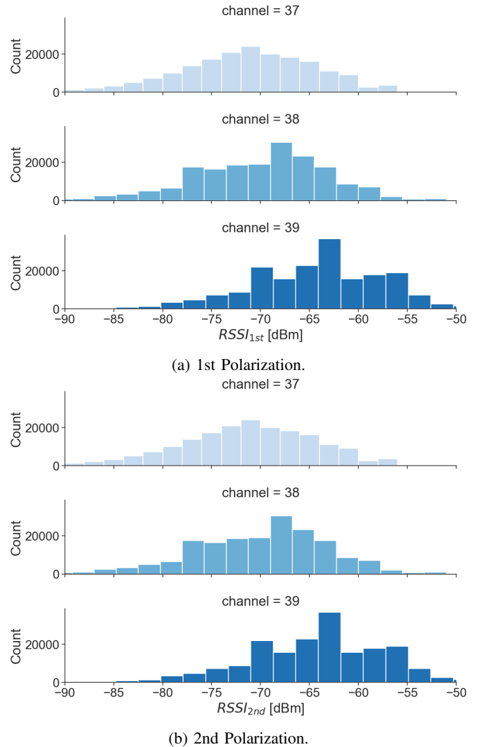
Fig. 10: RSSI distribution for three channels and two polarizations.
