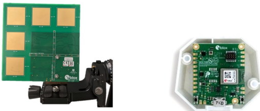
Fig. 4: The hardware kit used for the data collection: Anchor on the left, tag on the right.
