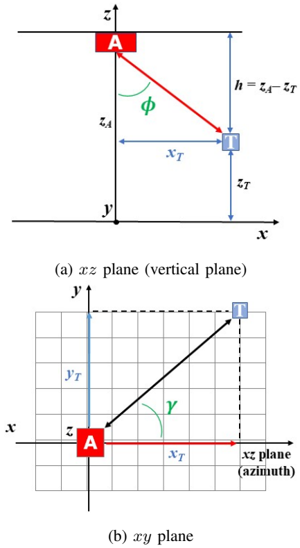
Fig. 13: Geometric representation of \phi and \gamma angles.
