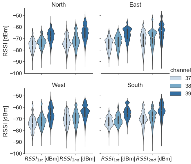
Fig. 11: RSSI distribution on 1st and 2nd polarization with four orientations (North, East, West, South) and three channels (37, 38, 39).
