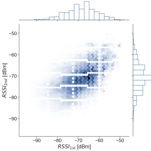
Fig. 9: Correlation between RSSI_{1st} and RSSI_{2nd} on the 1st and the 2nd polarization.
