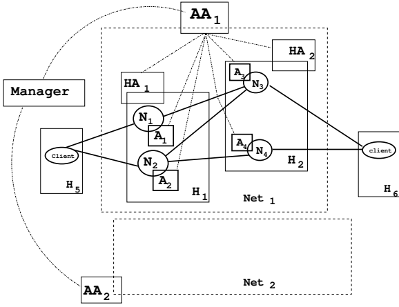
Figure 4. Lira infrastructure for the controlled network
