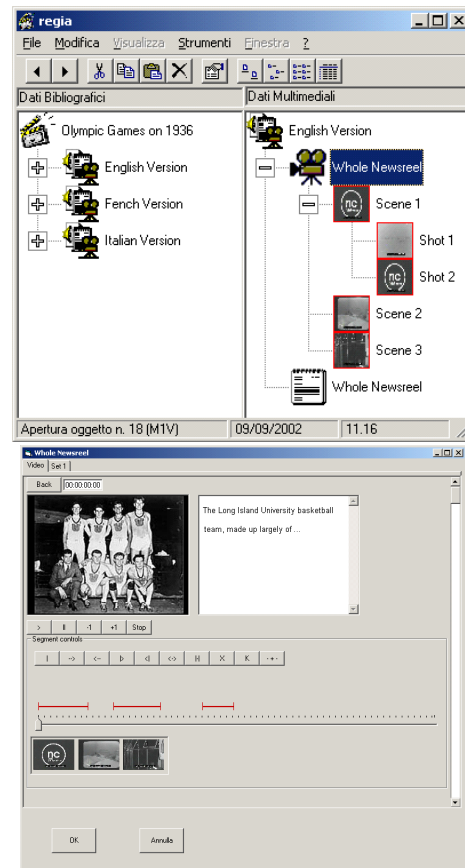
Fig. 2. A screenshot of the Metadata Editor. Document structure (above), and Expression editing tool (below).
