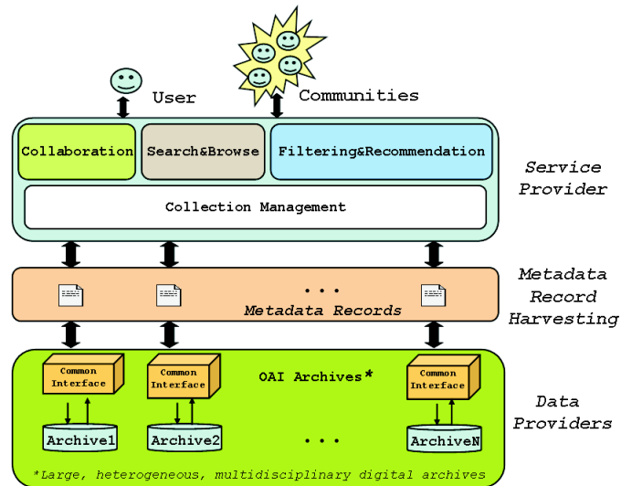
Figure 1: Logical view of CYCLADES.
