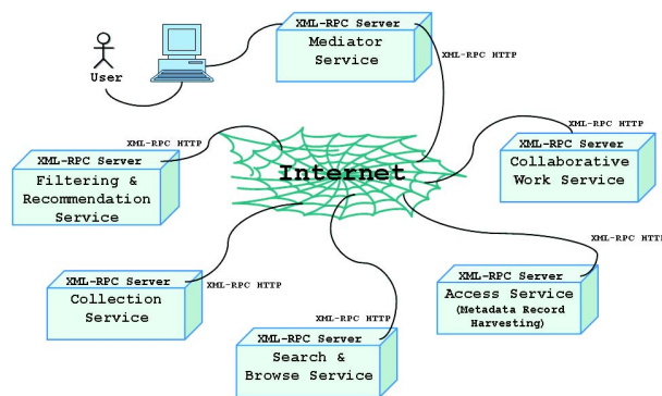
Figure 6: Architecture.
