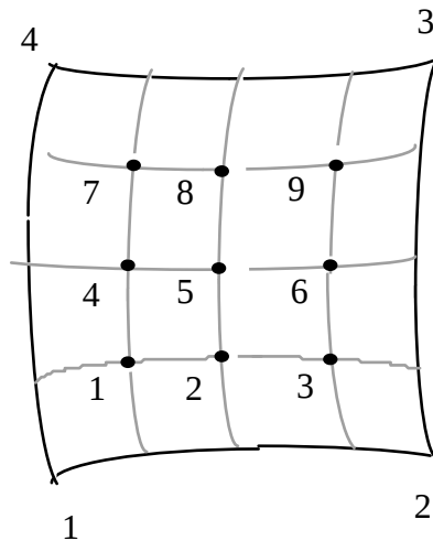
Figure 4.2 Integration points of elements 4.
