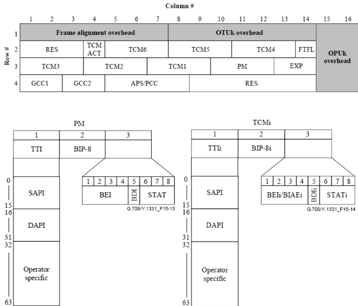
Figure 22: ODU overhead
