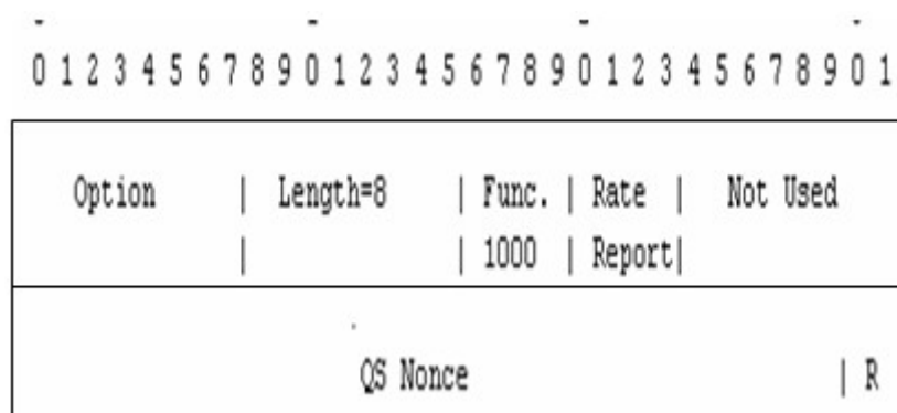
Figure 43: QS request header
