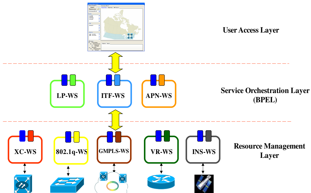
Figure 50: UCLP architecture overview
