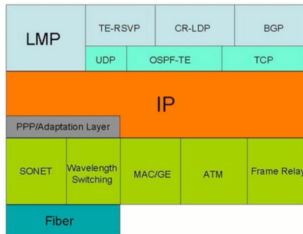
Figure 27: GMPLS protocol architecture
