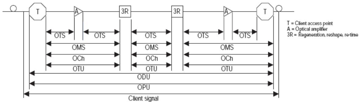
Figure 19: OTN layer termination points
