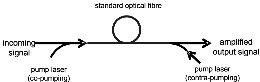
Figure 11: Raman amplification
