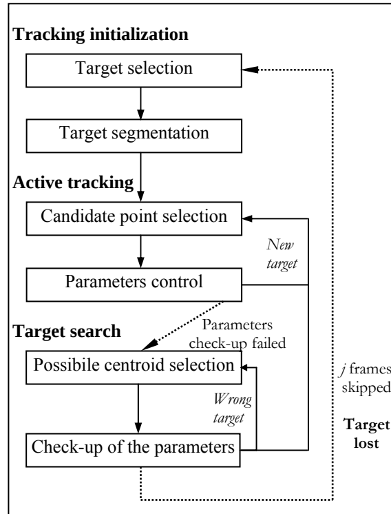
Fig. 9. Block diagram of the tracking algorithm
