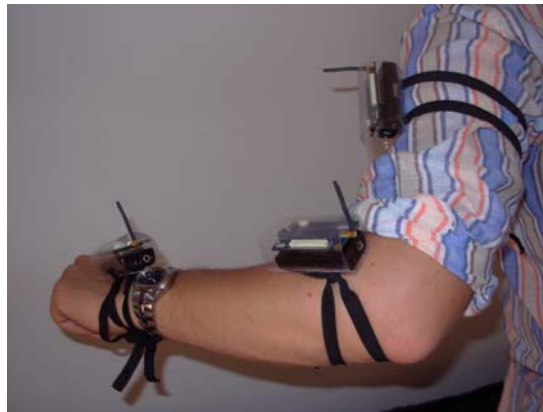
Figure 4. A detail of the body area sensor network.
