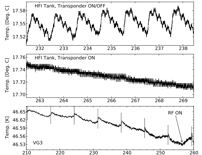
Fig. 7. A zoom of a seven day period on the temperature of a Helium tank is shown before (top panel) and after (middle panel) the RF transponder was left permanently on (see also Fig. 7), and illustrates the reduction in the daily temperature variations achieved by this operation. Smaller variations remain, due to thermal cycling of other elements (in this case the LFI Data Processing Unit), and are clearly visible in the middle panel. The bottom panel shows the typical effect of weekly updates of the operational parameters of the Sorption Cooler (marked as vertical lines) on the temperature of the third V-groove.
