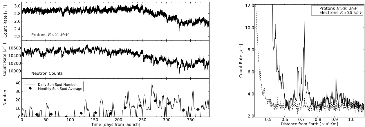
Fig. 8. The top left panel shows the time evolution of an SREM measure (TC1, Buehler et al. (1996)) which is sensitive to high-energy protons. The levels shortly after launch are also indicated (on the right), showing the passage through the van Allen radiation belts, characterised by very high count levels. The bottom panel (on the left) shows the corresponding evolution of the sunspot number, indicating the slow transition of the solar cycle out of its current minimum. A monitor of high-energy neutrons (in this case located at McMurdo station, data courtesy of Bartol Research Institute), presented in the middle panel, traces the corresponding decrease in the flux of Galactic cosmic rays as the Sun becomes more active.
