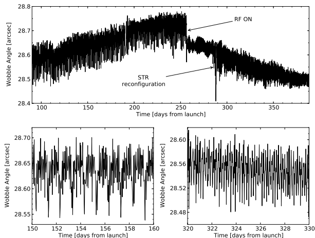
Fig. 10. Top: evolution of the measured offset between the principal axis of inertia and the geometric axis of the satellite (one point is plotted for each dwell period of approximately 50 minutes). The time variations observed are not real changes in the offset angle, but are instead due to thermoelastic deformations in the panel that supports the star trackers. Bottom: zooming in on short periods of time before (left) and after (right) the RF transponder was turned permanently on, reveals periodic variations (before, dominated by the daily RF On-Off switching; after, dominated by thermal control cycling of nearby units with typically one hour periodicity).
