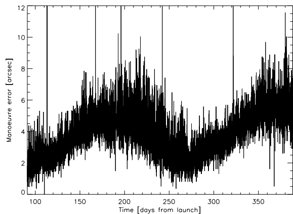
Fig. 12. The difference between the achieved and commanded pointing after each 2' manoeuvre, which is correlated with the duration of the previous dwell (see text). The vertical lines correspond to the very few occasions when the manoeuvre sequence did not execute as planned, resulting in anomalously high pointing errors.
