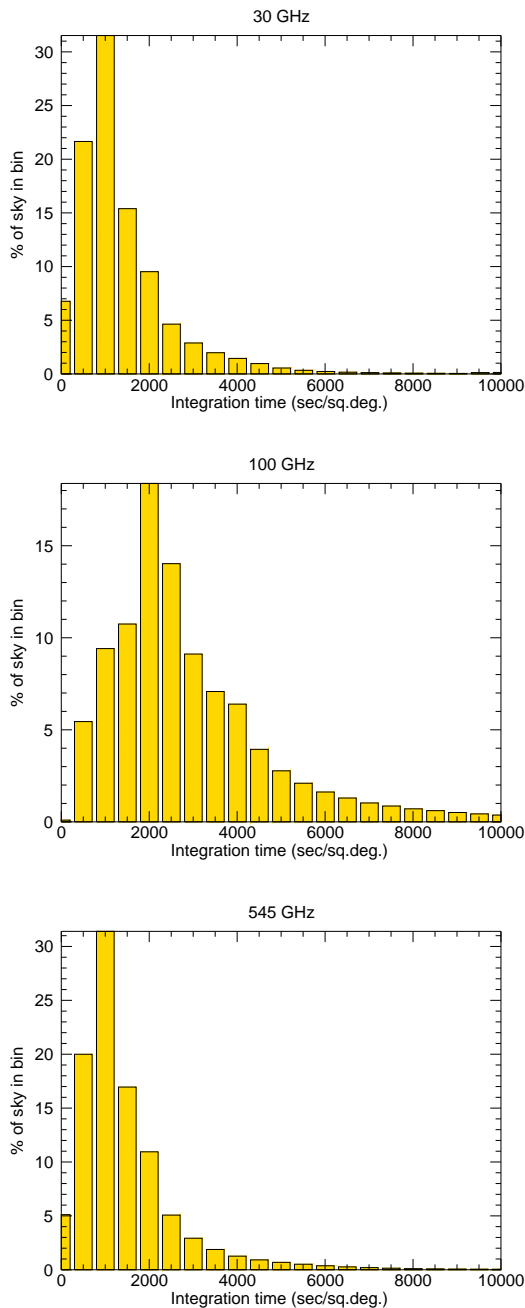
Fig. 5. Histograms of integration time (in \text{s deg}^{-2} ) cumulated for all detectors at 30 GHz (top panel), 100 GHz (middle panel), and 545 GHz (bottom panel). Characteristic coverage quantities are listed in Table 1.
