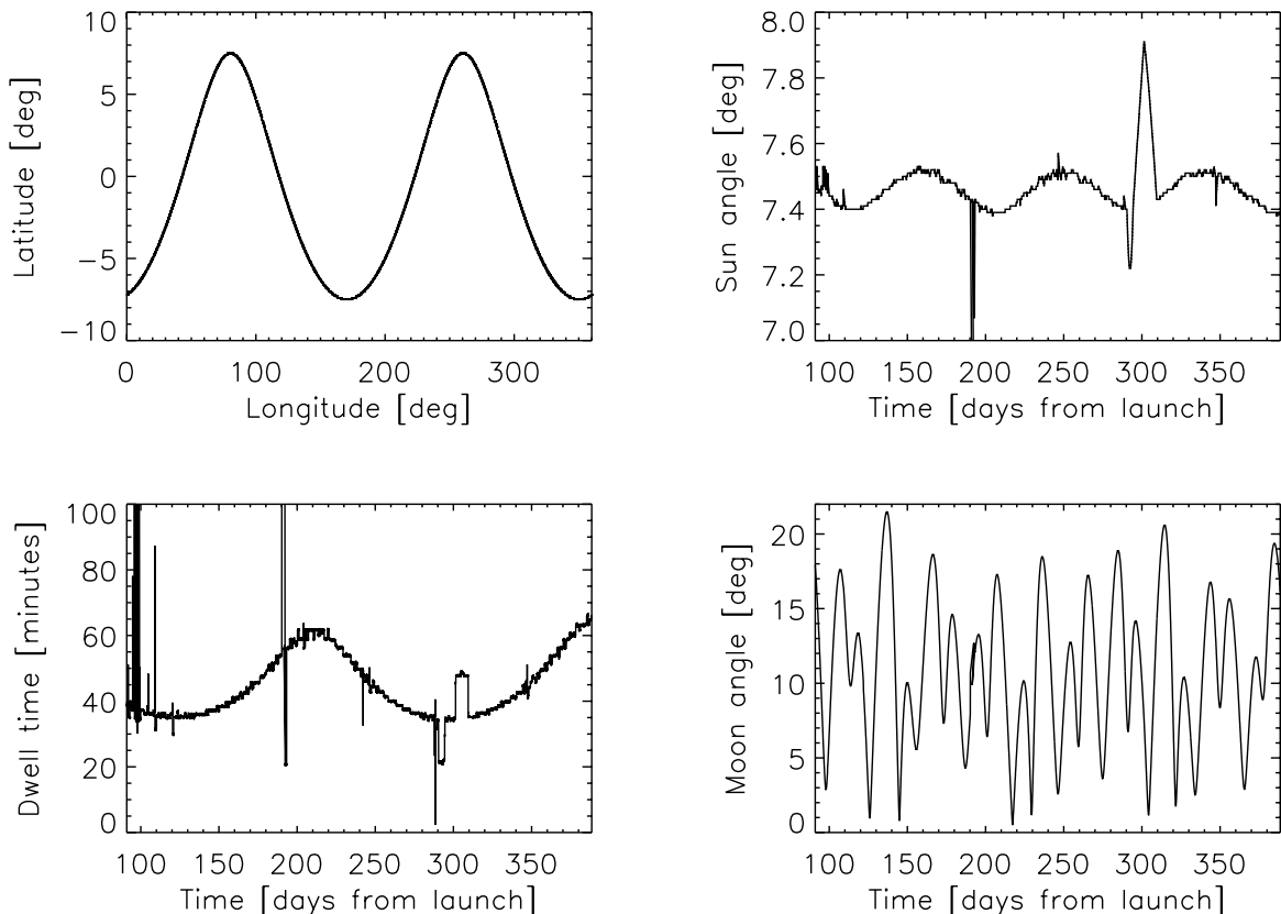
Fig. 3. Top left: the path of the spin axis of Planck (in Galactic latitude and longitude) over the period 13 August 2009 to 6 June 2010. The evolution of the dwell time (bottom left) and of the solar aspect angle (top right) are shown during the same period. The “day Planck stood still” (day 191) and the period of acceleration/deceleration during observations of the Crab (between days 291 and 310) are clearly visible in both plots. Bottom right: the evolution of the angle between the Moon and the field-of-view of the telescope.
