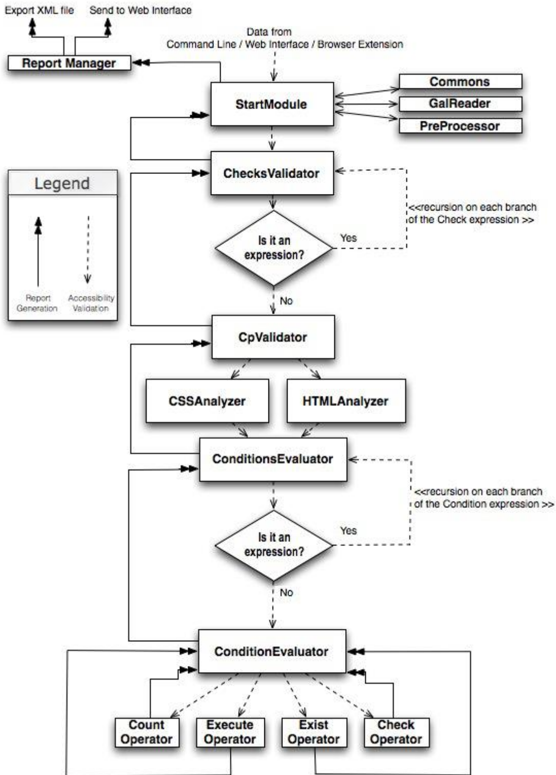
Figure 4 MAUVE Validator's Evaluation Logic.
