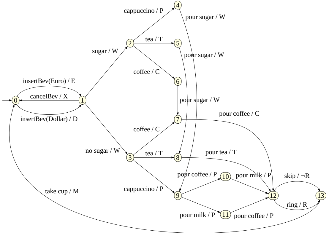
Figure 7: FTS of beverage component
