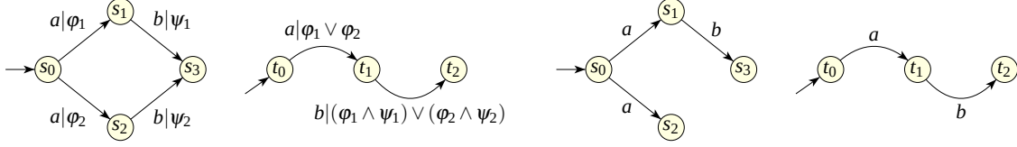
Figure 3: Bisimilar FTS assuming \phi_1 \wedge \phi_2 \Rightarrow (\psi_1 \Leftrightarrow \psi_2) and non-bisimilar LTS
