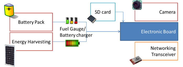
Fig. 3 Architecture of the smart camera
