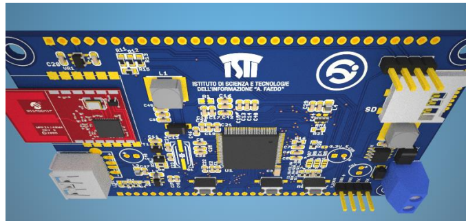
Fig. 4 Layout of the smart camera board
