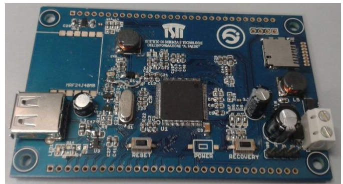
Fig. 8 The smart camera main electronic board
