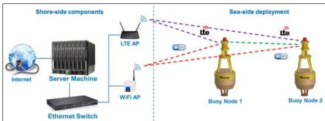
Figure 5. UTH's Deployment Architecture
