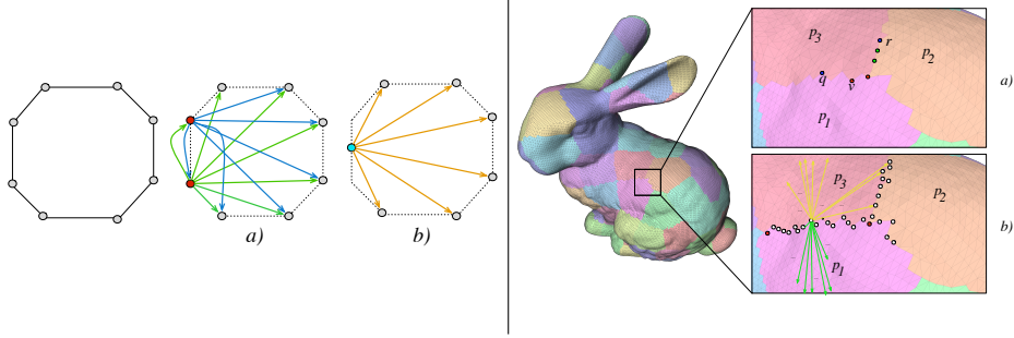
Fig. 4. Left: Pruning of two nodes: a) Two red vertices are selected for pruning. b) Pruning produces a new dummy node; Right: a) An example of a pair of nodes eligible for pruning (green) and two pairs not eligible (blue and red). b) An example of a border vertex and its |Bv| \times |Bv| edges in both the patches it is contained. To have a clear picture, edges are only sketched.
