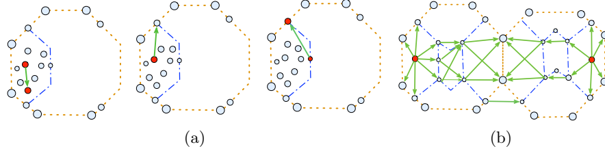
Fig. 6. a) Different cases of geodesic computation between vertices that belong to the same patch at the final level; b) The set of arcs enabled for Dijkstra shortest path computation for the general case.
