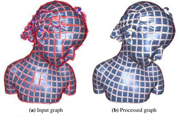
Figure 14: The position field and integer jumps generated by the second stage of our optimization pipeline are already in a form that is very close to the final output mesh: (a) shows a visualization of the position field, where zero integer jumps are connected by a blue line, and red lines indicate unit jumps. We collapse clusters of blue links into the vertices of the output mesh, shown in (b), and extract polygons from the resulting graph.
