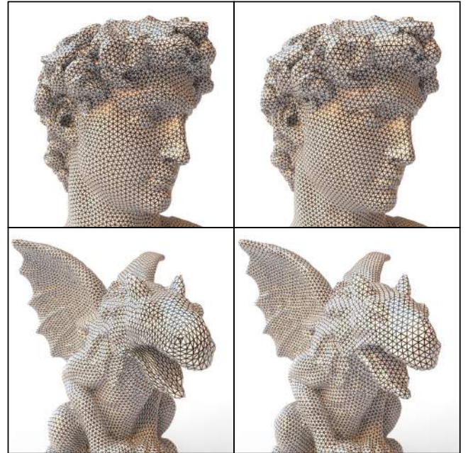
Figure 16: Triangle meshing comparison: [Surazhsky et al. 2003] (top left), [Pietroni et al. ] (bottom left) and our results on the right. Note that our meshes are better aligned to the shape features.
