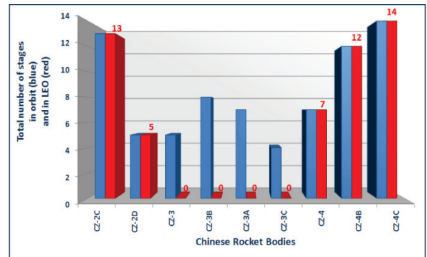
Fig. 12: Distribution among rocket types and orbital regimes of the upper stages launched by China 2 .
