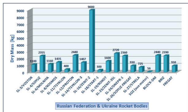
Fig. 7: Dry masses of the upper stages launched by the Russian Federation and Ukraine 2 .
