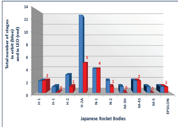
Fig. 14: Distribution among rocket types and orbital regimes of the upper stages launched by Japan 2 .
