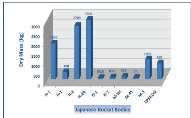
Fig. 13: Dry masses of the upper stages launched by Japan 2 .
