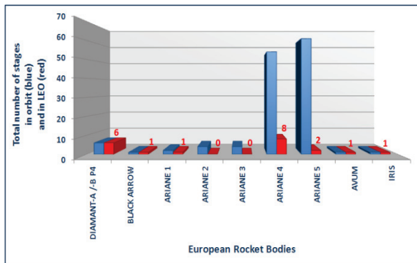
Fig. 10: Distribution among rocket types and orbital regimes of the upper stages launched by Europe 2 .
