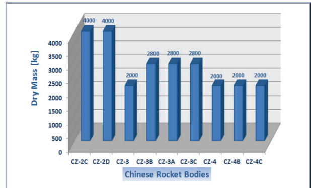
Fig. 11: Dry masses of the upper stages launched by China 2 .
