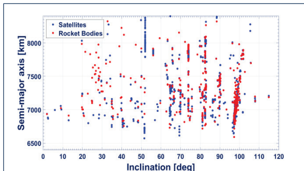
Fig. 1: Distribution of intact satellites and rocket bodies fully residing in LEO as a function of semi-major axis and inclination (January 7, 2015). The Earth's equatorial radius is about 6378 km.
