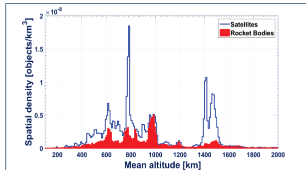
Fig. 2: Spatial density in LEO of intact satellites and rocket bodies (January 7, 2015).
