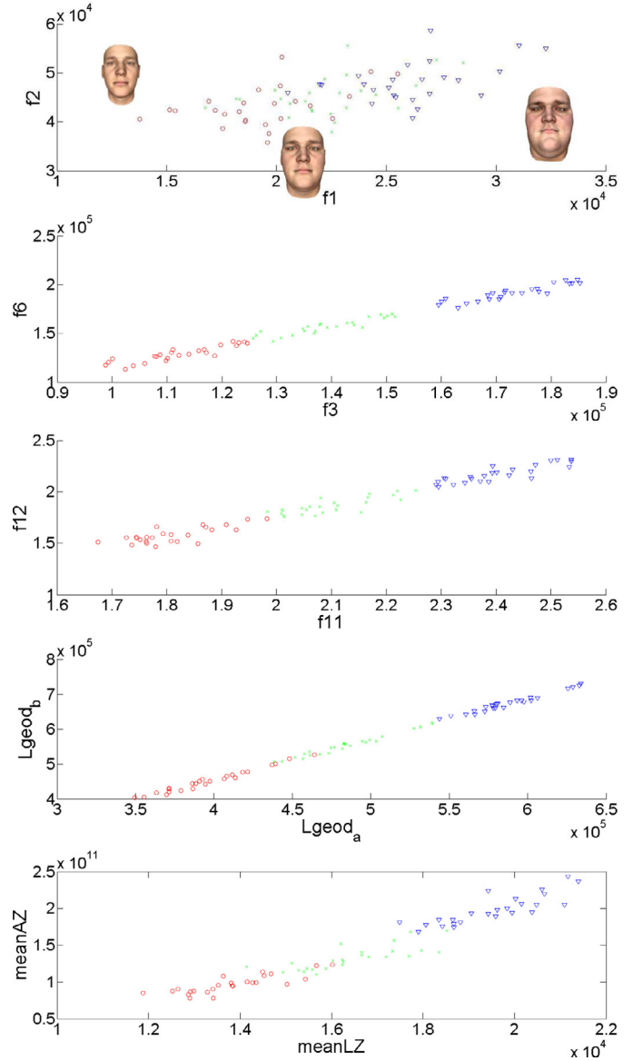
Fig. 16. Scatter plots for the subjects belonging to three groups of fatness: level 1, in red, level 5, in green, and level 10, in blue) in the embedding space given by the features f1 and f2 , f3 and f6 , f11 and f12 , Lgeod_a and Lgeod_b , meanLZ and meanAZ . (For interpretation of the references to colour in this figure legend, the reader is referred to the web version of this article).
