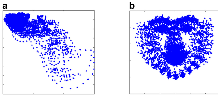
Fig. 21. Landmarks distribution (a); landmarks distribution after GPA alignment (b).
