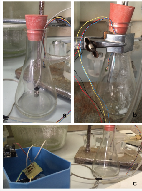
Figure 9. a) Experimental setup for gas sensors tests. b) The humidity is kept constant by means of a saturated solution of NaCl placed on the bottom of the vial. c) The data stream from sensors is read by an Arduino board.
