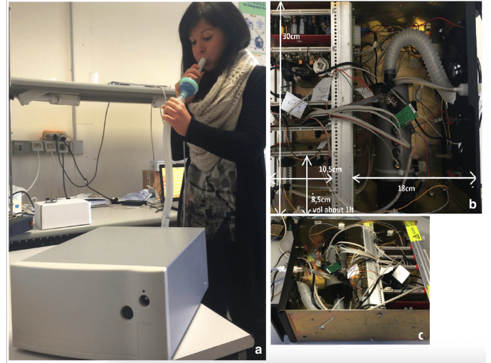
Figure 1. a) Wise Sniffer first prototype's hardware. b) and c) show its internal configuration.
