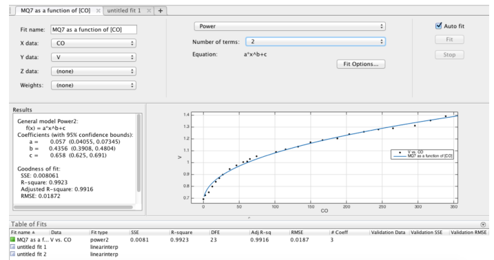
Figure 7. The relationship between MQ7 sensor's output and well-known CO concentrations is plotted. A power model is used for fitting curve. Measurement conditions: 25.98C, 65.3%RH
