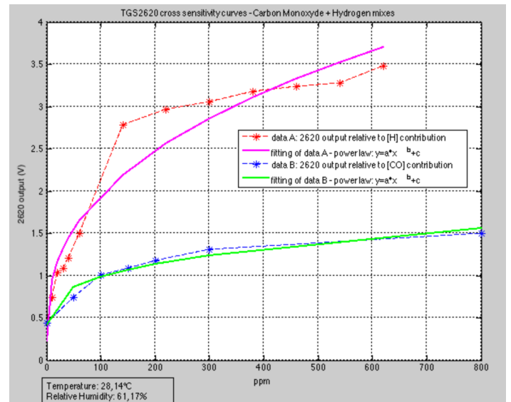
Figure 8. The contributions of well-known carbon monoxide and hydrogen gaseous mixes on TGS2620 sensor's output. It can be noted that such sensor is much sensitive to hydrogen than to carbon monoxide, especially at lower concentrations.
