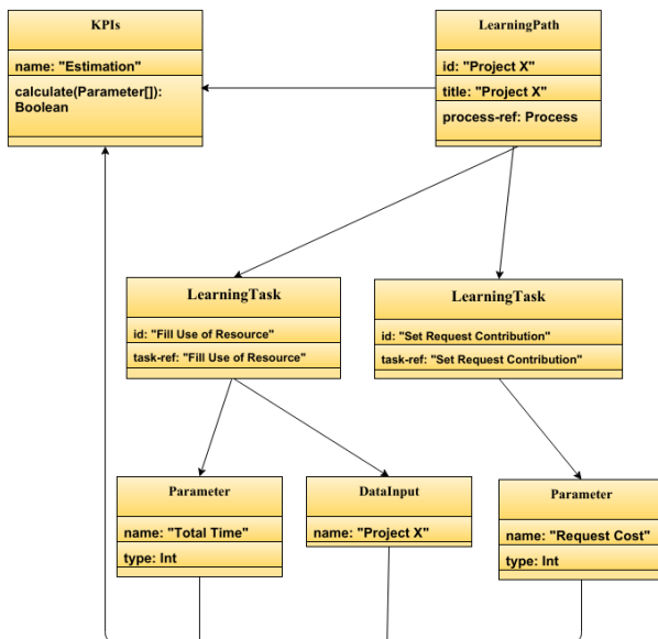
Figure 4: Learning Path Specification- Periodic Budgeting Report
