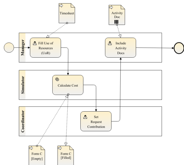
Figure 3: Example Process- Periodic Budgeting Report
