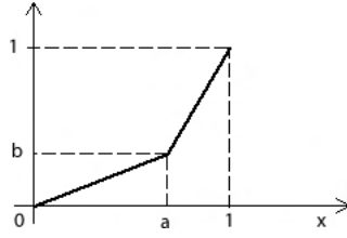
Figure 5: Linear modifier lm(a, b) .
