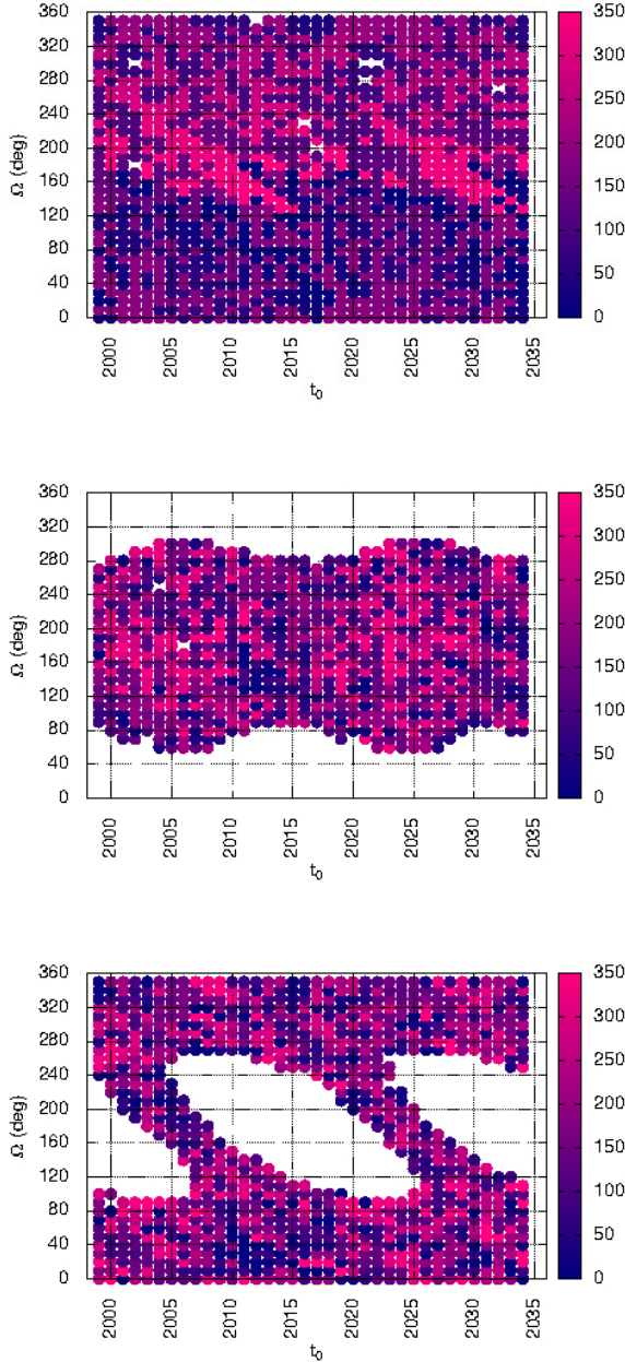
Figure 3. As a function of the initial epoch t_0 and longitude of ascending node \Omega we show, for the eccentricity growth scenario, for Galileo, the value of argument of pericenter in degrees (color bar) which ensures a re-entry. Top: nominal initial inclination; middle initial inclination decreased by 1^\circ ; Bottom initial inclination increased by 1^\circ .
