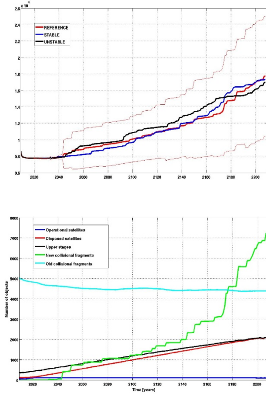
Figure 4. Top panel: Effective number of objects between 15000 and 35000 km, larger than 5 cm in the three scenarios: Reference (thick red line), Stable (blue line) and Unstable (black line). The thin red lines show the \pm 1 sigma of the MC averaging in the Reference case. Bottom panel: Effective number of objects between 15000 and 35000 km, larger than 5 cm divided by type: operational satellites (blue), disposed satellites (red), upper stages (black), old collisional fragments (cyan) and new collisional fragments (green).
