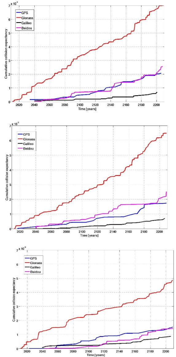
Figure 7. Cumulative collision expectancy for operational satellites belonging to the four GNSSs in the Reference (Top panel), Stable (middle panel) and Unstable (bottom panel) scenarios. The red line refers to Glonass, the blue line to GPS, the magenta line to Beidou and the black line to Galileo
