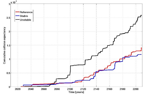
Figure 8. Comparison of the cumulative collision expectancy for non-operational Galileo satellites against all other GNSS operational satellites in the three scenarios: Reference (red), Stable (blue) and Unstable (black). See text for details.
