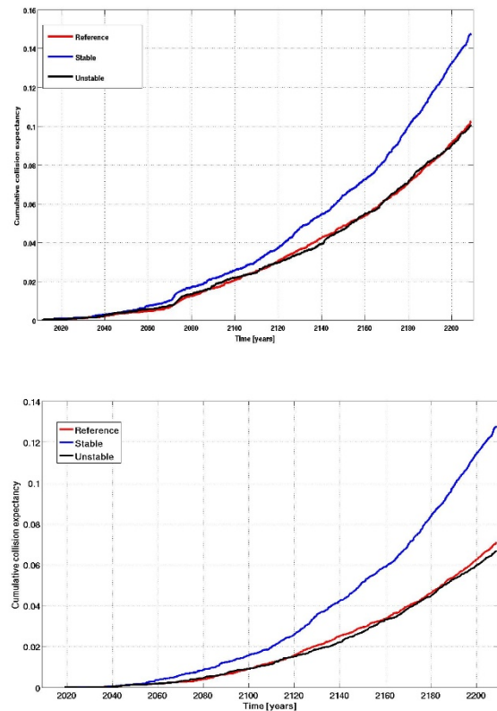
Figure 6. Top panel: cumulative collision expectancy for objects belonging to the GNSSs (both operational and disposed) in the three main scenarios: Reference (red), Stable (blue) and Unstable (black). Bottom panel: cumulative collision expectancy for non-operational objects belonging to the GNSSs against every other non-controlled object (i.e., other GNSSs non-operational, upper stages, fragments, MRO,...). See text for details.
