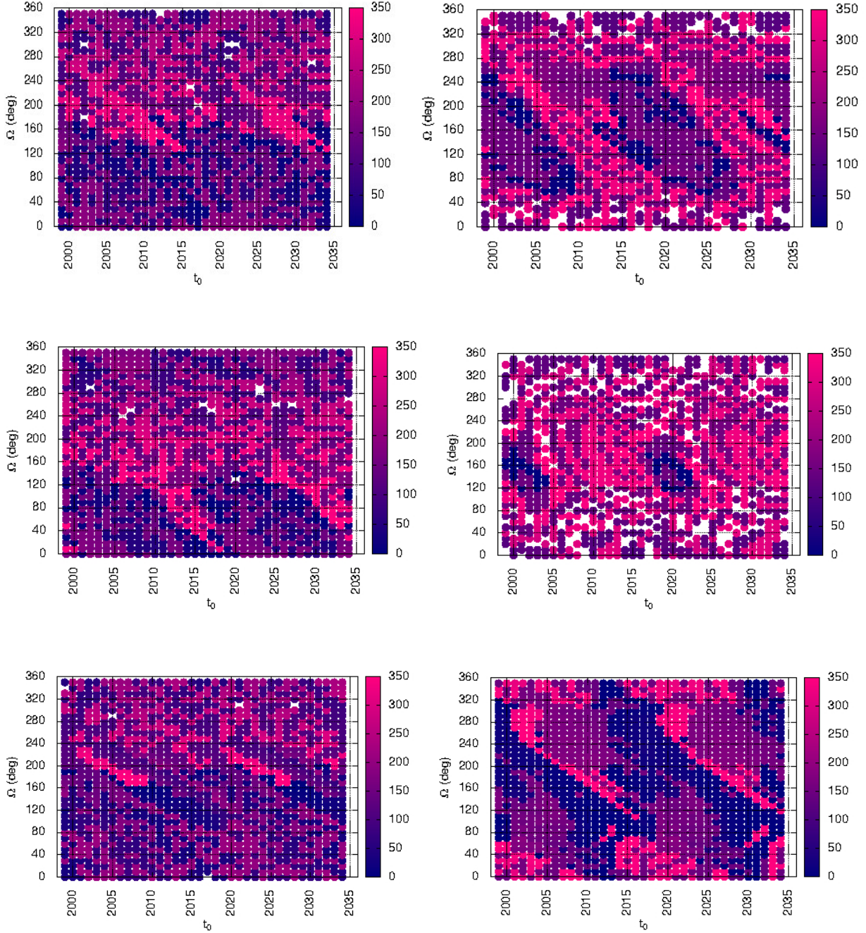
Figure 1. As a function of the initial epoch t_0 and long. of asc. node \Omega we show, in the graveyard orbit scenario for Galileo (left) and GLONASS (right), the value of \omega in degrees (color bar) which ensures that the eccentricity will not exceed 0.02 in 200 years. Whenever there exist two values, we represent the one corresponding to the minimum ecc. growth. Top nominal initial inclination; middle initial i decreased by 1^\circ ; bottom: initial i . increased by 1^\circ .
