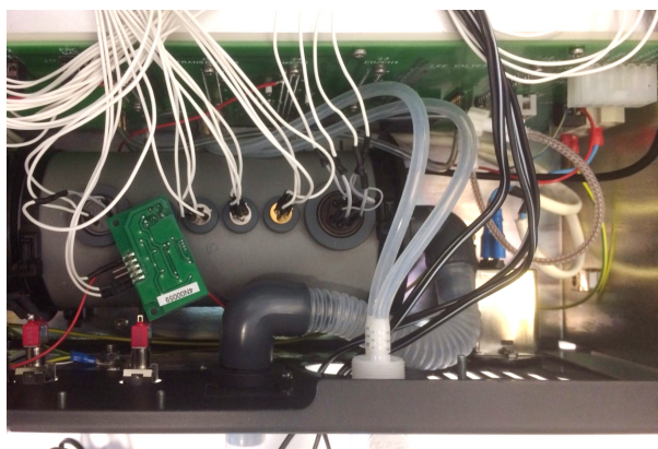
Figure 2. Wize Sniffer's gas sampling chamber detail
