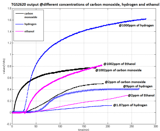
Figure 7. TGS2620 output when well-known concentrations of \text{CO} , \text{H}_2 and \text{C}_2\text{H}_6\text{O} were separately injected into the vial.
