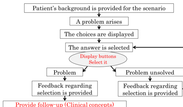
Figure 3. E-learning Flow
