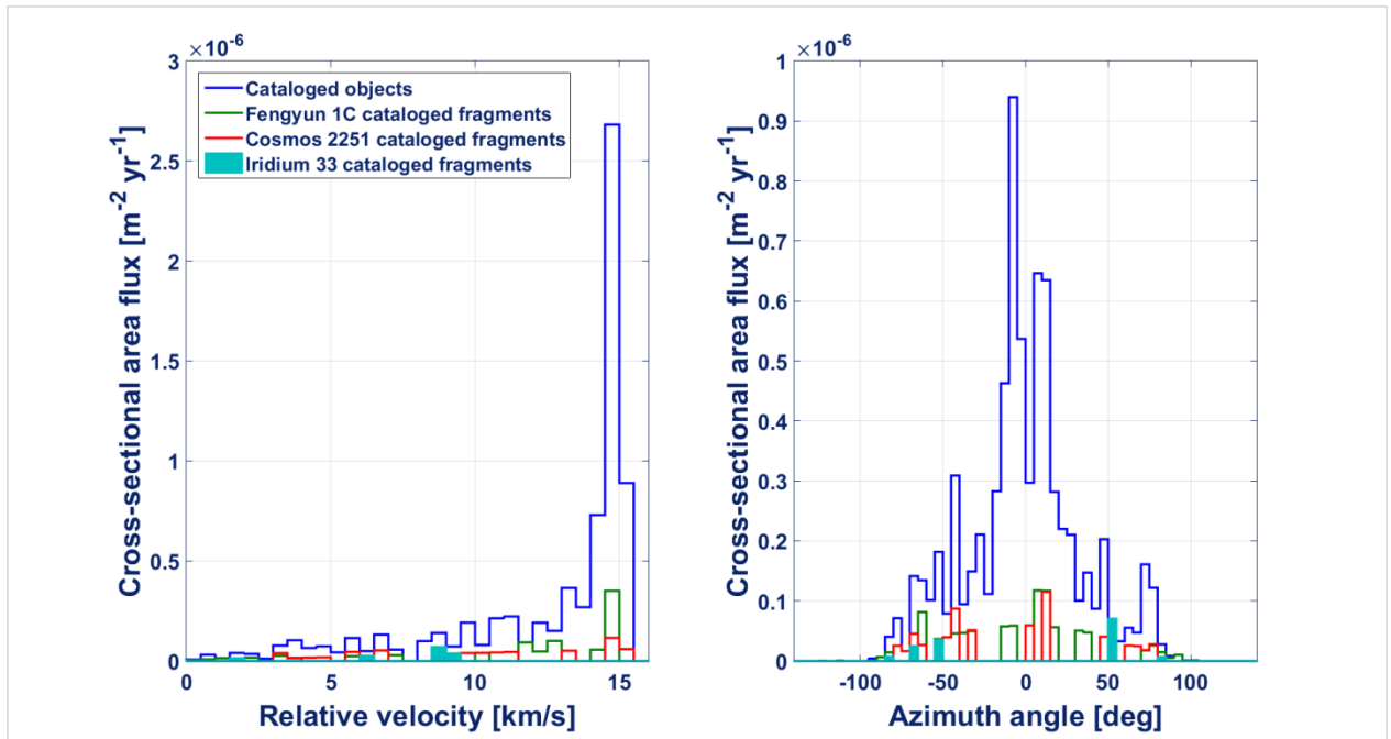
Fig. 16: Relative velocity and directional flux of cataloged objects (8 June 2016) on the COSMO-SkyMed constellation.
