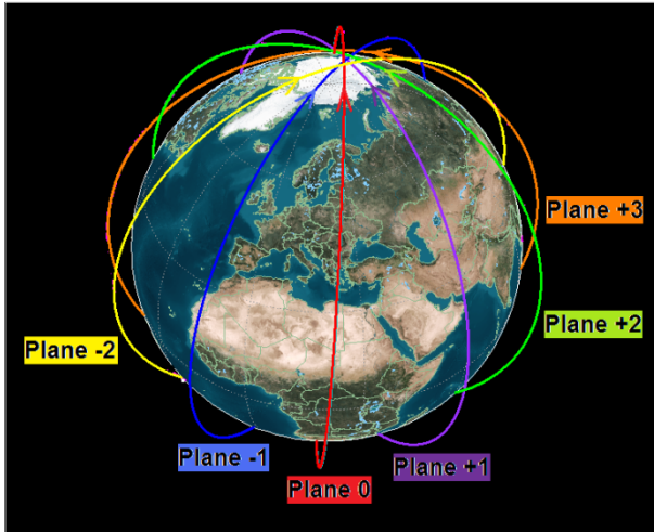
Fig. 8: Distribution of the orbit planes of the Iridium constellation, referred counterclockwise with respect to the Iridium 33 original plane (Plane 0).
