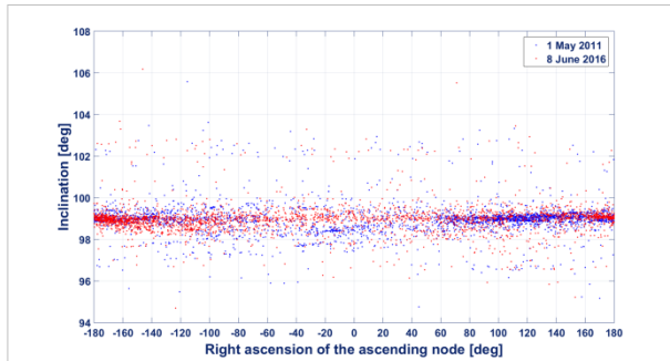
Fig. 5: Evolution of the nodal distribution of the Fengyun 1C debris cloud.
