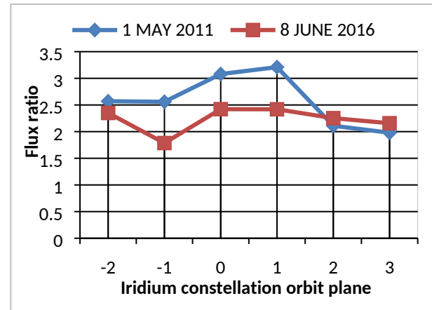
Fig. 9: Ratio of the total flux of cataloged objects to the background flux obtained by excluding the Fengyun 1C, Cosmos 2251 and Iridium 33 debris (in the ordinate) as a function of the Iridium constellation orbit planes.
