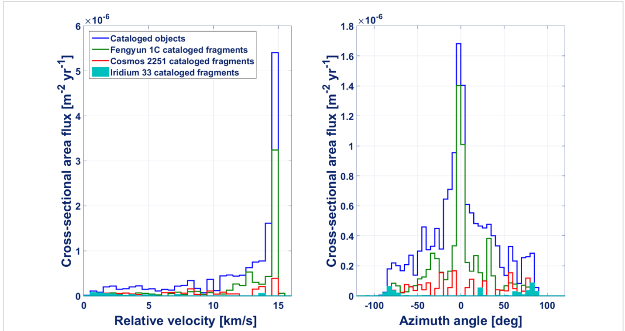
Fig. 12: Relative velocity and directional flux of cataloged objects (8 June 2016) on the Iridium operational plane 0.
