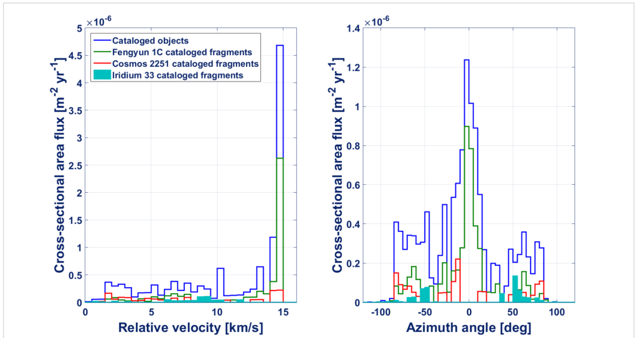
Fig. 14: Relative velocity and directional flux of cataloged objects (8 June 2016) on the Iridium operational plane +2.
