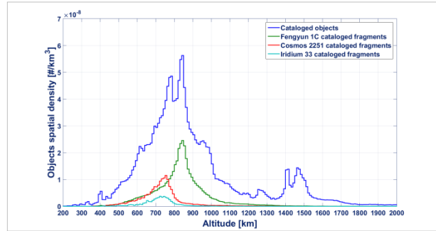
Fig. 3. Spatial density of cataloged objects in LEO with publicly available TLEs on 8 June 2016, showing also the Fengyun 1C, Cosmos 2251 and Iridium 33 debris clouds.
