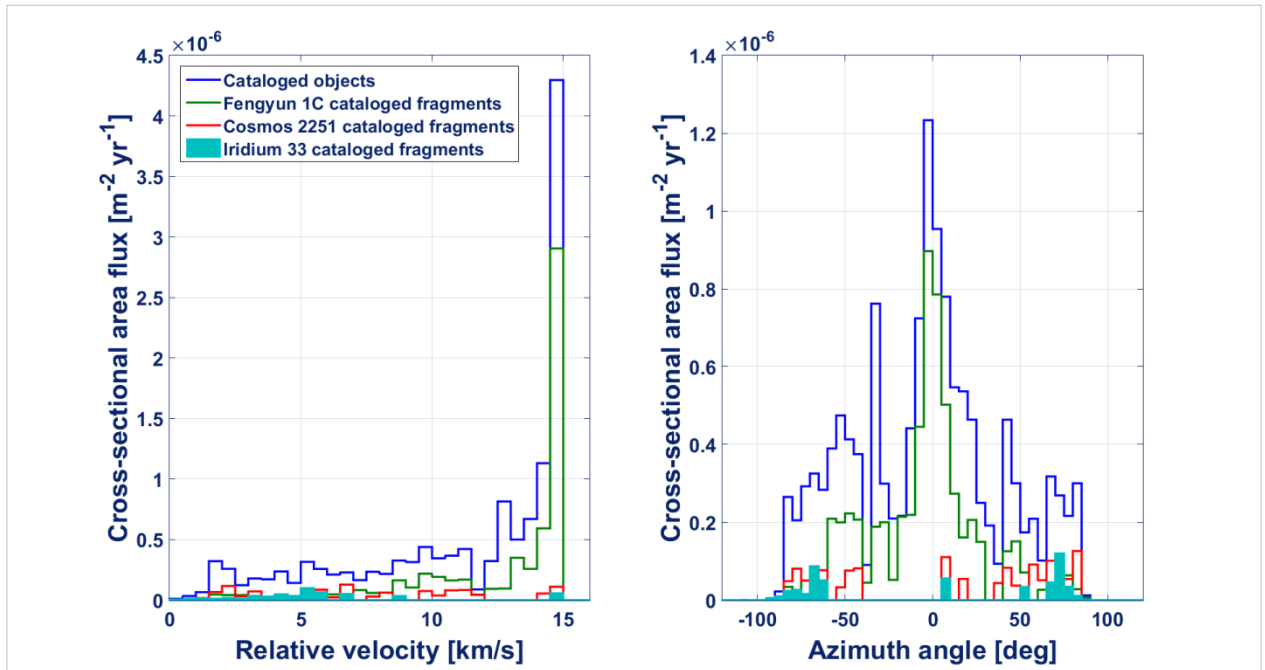
Fig. 13: Relative velocity and directional flux of cataloged objects (8 June 2016) on the Iridium operational plane +1.
