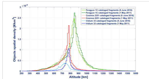
Fig. 4. Evolution of the spatial density of the cataloged debris belonging to the Fengyun 1C, Cosmos 2251 and Iridium 33 debris clouds during about five years, from 1 May 2011 to 8 June 2016. The discovery and cataloging of new fragments during that period were more than compensated by the secular orbital decay induced by thermospheric drag.
