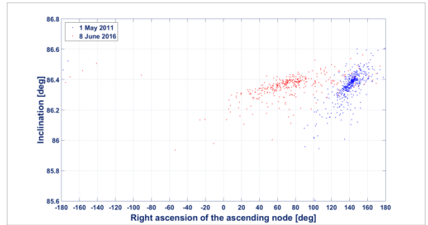
Fig. 7: Evolution of the nodal distribution of the Iridium 33 debris cloud.
