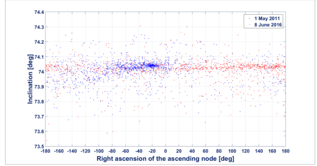
Fig. 6: Evolution of the nodal distribution of the Cosmos 2251 debris cloud.
