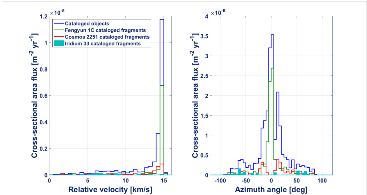
Fig. 10: Relative velocity and directional flux of cataloged objects (8 June 2016) on the Iridium operational plane -2. The azimuth angle is measured clockwise from the projection of the velocity vector in the target centered horizon plane. Most of the flux exhibits elevation angles < 5 deg with respect to the local horizon.
