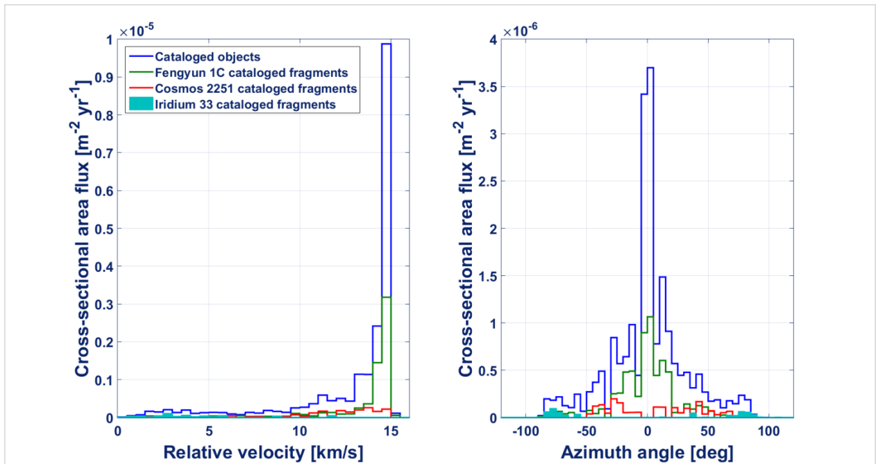
Fig. 11: Relative velocity and directional flux of cataloged objects (8 June 2016) on the Iridium operational plane -1.
