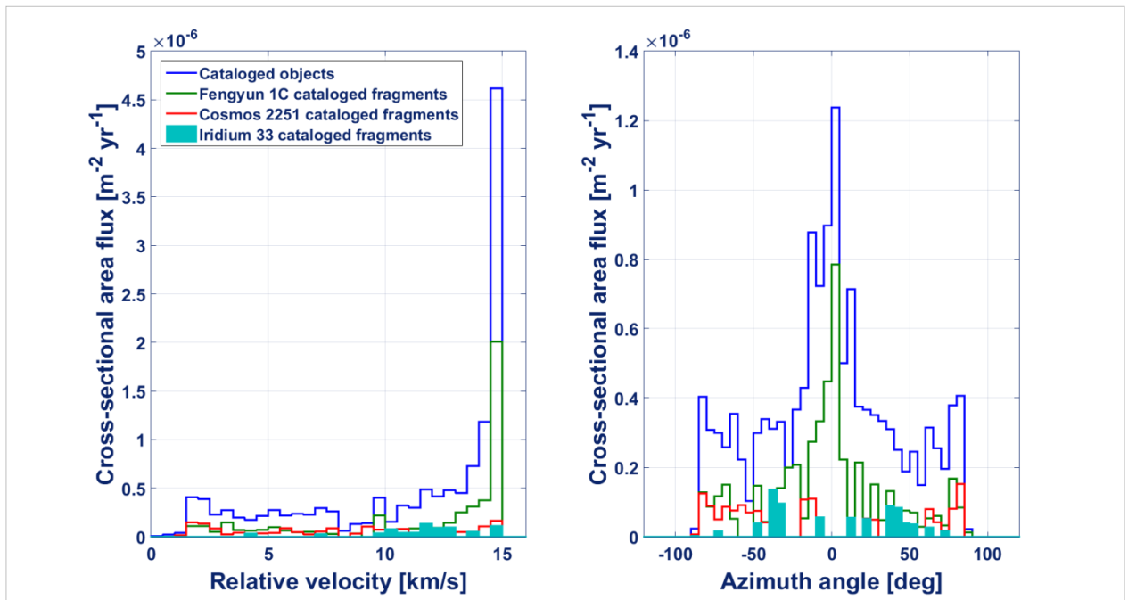
Fig. 15: Relative velocity and directional flux of cataloged objects (8 June 2016) on the Iridium operational plane +3.
