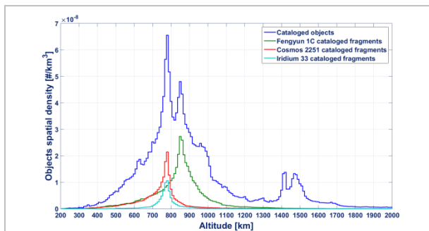
Fig. 2. Spatial density of cataloged objects in LEO with publicly available TLEs on 1 May 2011, showing also the Fengyun 1C, Cosmos 2251 and Iridium 33 debris clouds.
