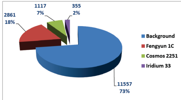
Fig. 1. Cataloged objects in orbit with publicly available TLEs (15,890), as of 8 June 2016, showing the contribution of the Fengyun 1C, Cosmos 2251 and Iridium 33 fragments.
