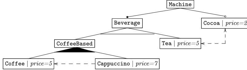
Fig. 3. Feature model of vending machine product line
