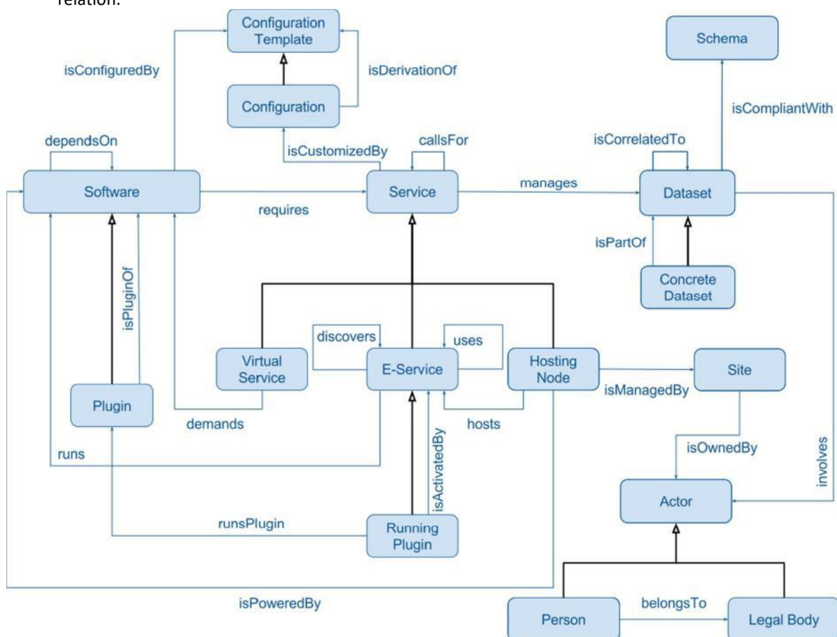
Fig. 2 Overview of gCube Model Resources and (isRelatedTo) Relations
