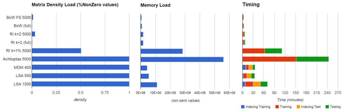
Figure 3: Reuters RCV1/RCV2 English and Italian (11,200-by-51,828 full training matrix size). Left: matrix density; center: memory load; right: execution time.
