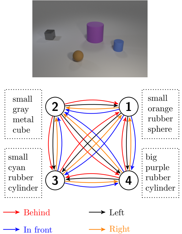
Fig. 1: CLEVR scene with associated scene graph.
