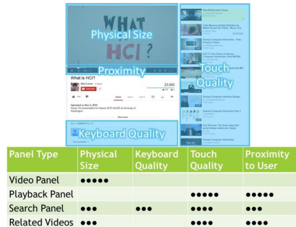
Fig. 14. How Panelrama [86] classifies the various user interface parts
