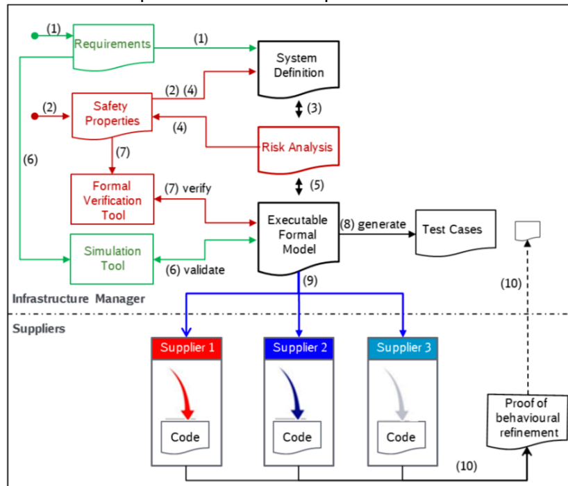
Figure 8 X2Rail2 Use case for formal development of systems with standardised interfaces
