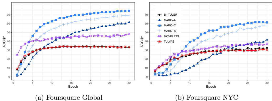
Figure 6.: Classification accuracy (ACC@1) over training time (Epoch) of compared approaches, considering the datasets without the POI identifiers.
