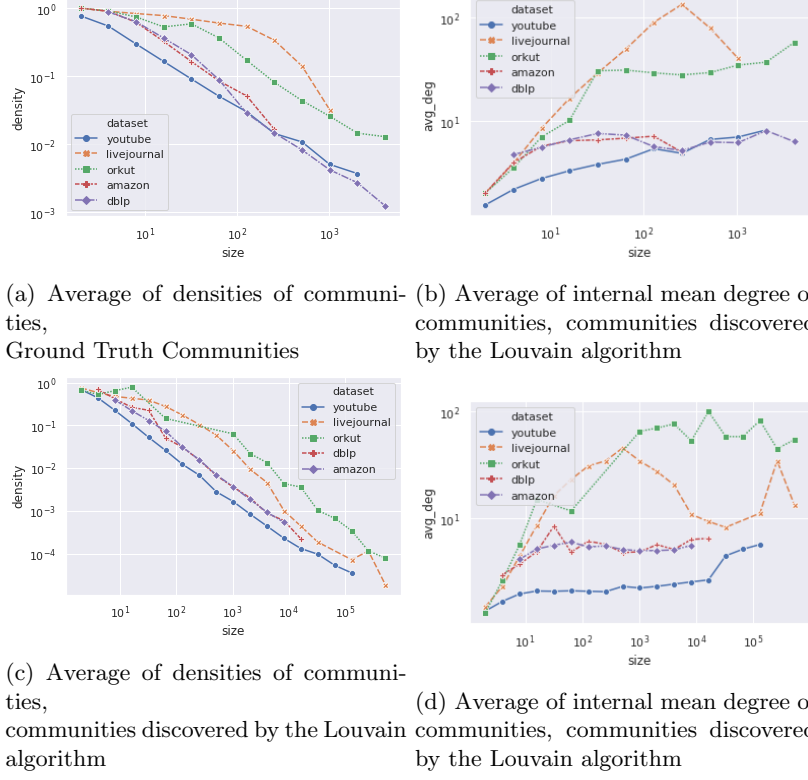
Figure 3: relation between densities/mean degrees of communities relatively to their size in several large networks with available ground-truth communities. We observe similar trends for most networks: density decreasing with size, average internal degree increasing with size.
