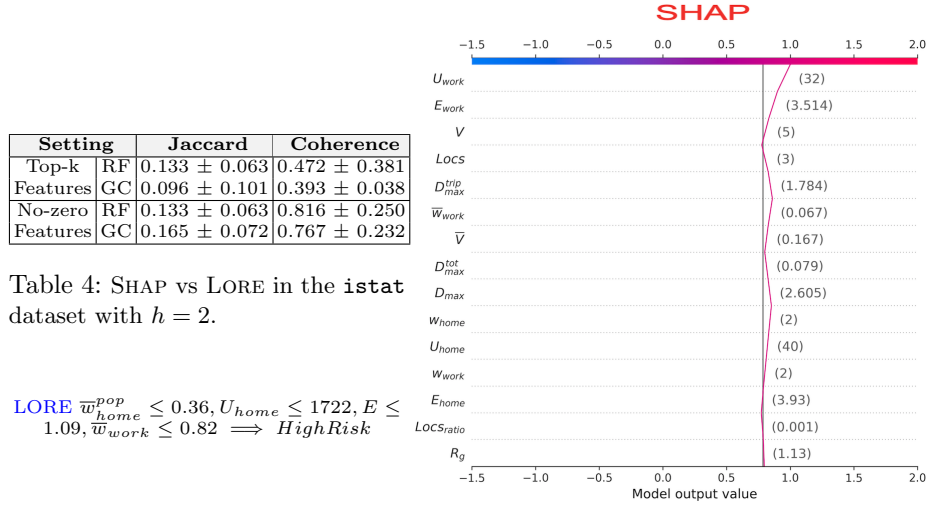
Fig. 2: SHAP vs LORE: Table 4 quantifies the similarity between the two explanations. SHAP visualization (right) and the LORE rule (left) represent the explanations for a specific record classified as high risk by GCForest.
