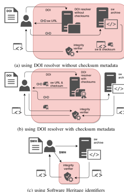
Figure 4. Trusted third parties (shown as rounded red boxes) for software artifact retrieval and verification in three different
