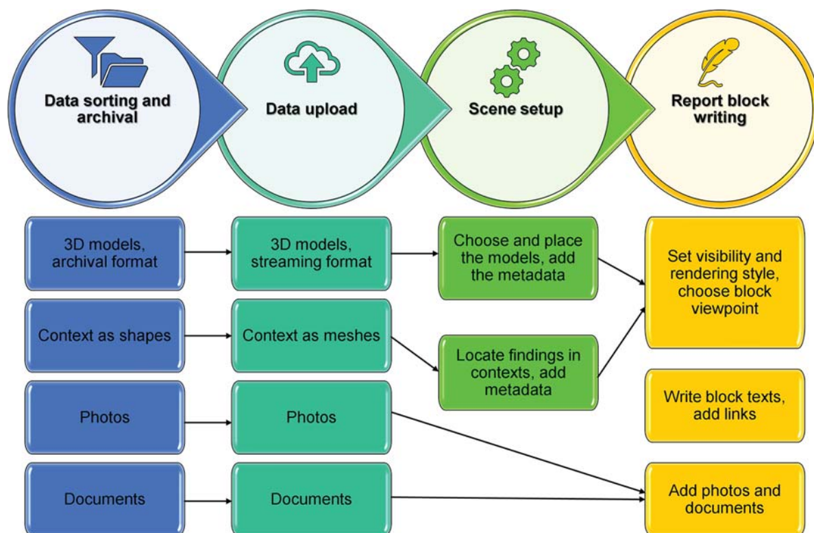
Figure 10. The representative scheme of the authoring workflow of the Interactive Reporting System; data is sorted and archived before uploading it in the system. Once the scene setup is complete, you can write the report blocks.
