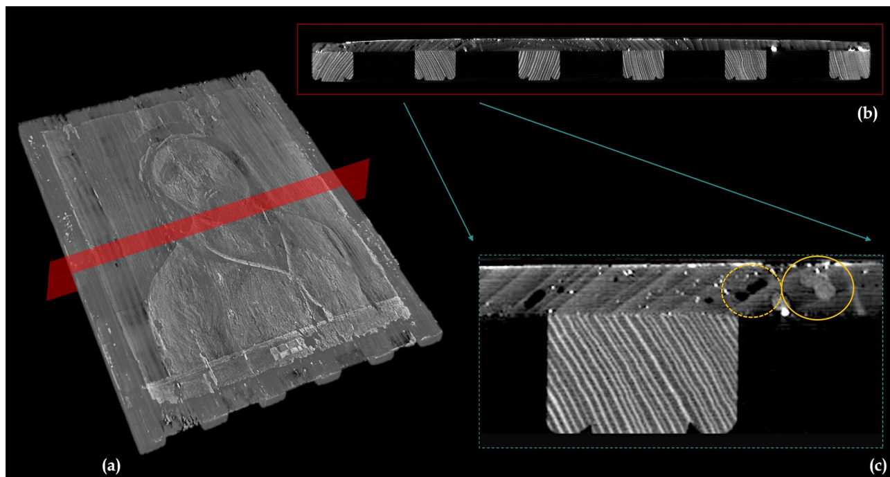
Figure 2. Tomographic analysis of the painting support. (a) 3D rendering of the entire tomographic volume and the virtual plane analysed (in red). (b) The corresponding tomographic slice shows the massive cradling, slim support, and extremely thin painting layers. (c) A detail of the previous section where several woodworm tunnels are visible, some are empty , and some have been filled with dust and wood residues (highlighted with dashed and continuous yellow circles).
